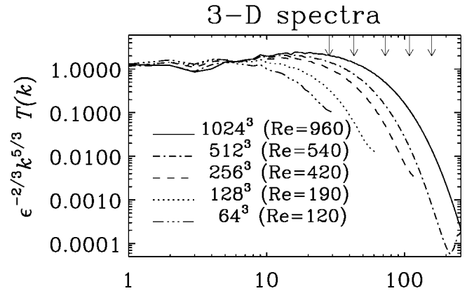
FIG. 4.—Total energy spectra compensated by \epsilon_T^{-2/3} k^{5/3} , where \epsilon_T is the rate of total energy dissipation. Spectra for different resolution are compared. The dissipation cutoff wavenumber, k_d = (\epsilon_T/\nu^3)^{1/4} , is indicated by short arrows at the top of the plot. The Reynolds number, \text{Re} = u_{\text{rms}}/\nu k_f , is given in the legend.
