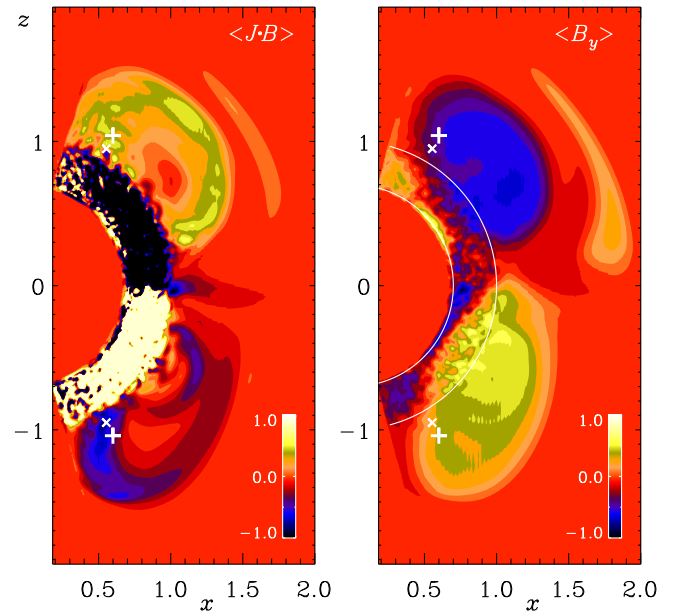
Figure 1. \langle \mathbf{J} \cdot \mathbf{B} \rangle_y (left) and \langle B_y \rangle_y (right) at t/\tau = 430 . The crosses and plusses mark positions at r/R = 1.1 and 1.2 and 90^\circ - \vartheta = \pm 60^\circ latitude, for which the \lambda^2 dependence is studied in Figure 2.
