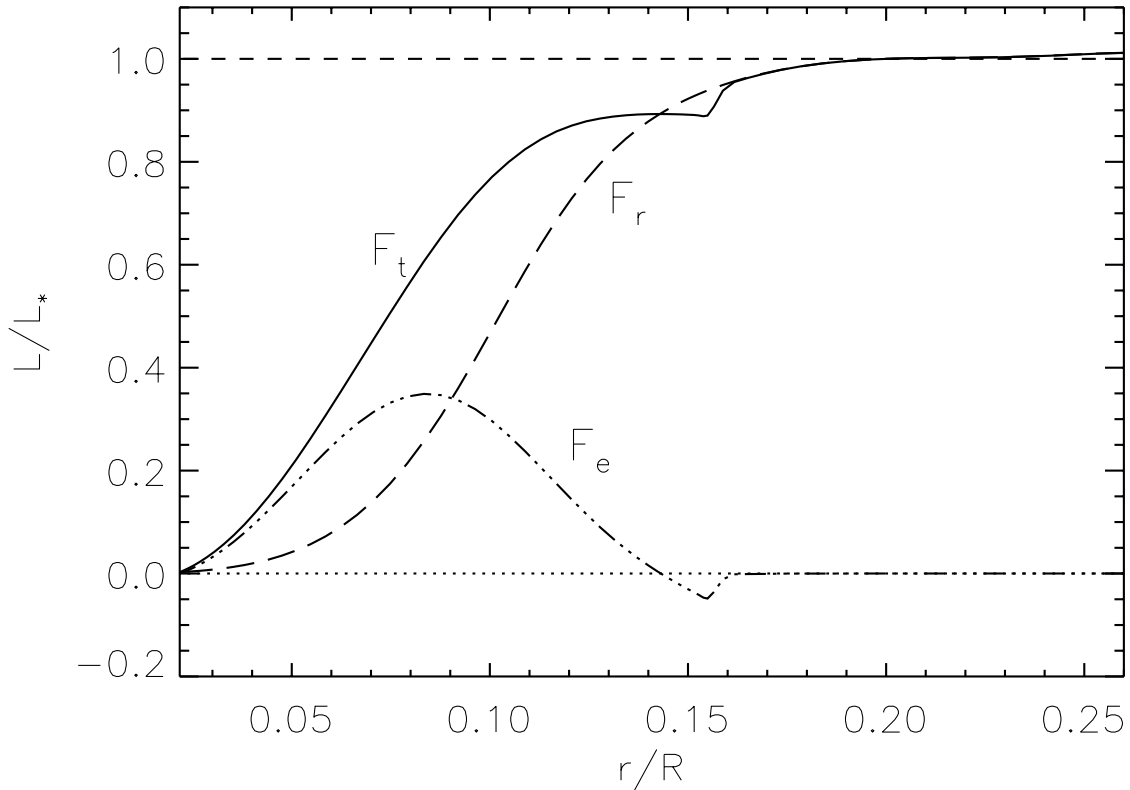
Fig. 5.— Time-averaged radial transport of energy within case C as a function of proportional radius, formed over an interval of about 180 days. Shown are the enthalpy flux F_e and the radiative flux F_r , together with their sum, the total flux F_t ; all quantities have been expressed as luminosities. The convective core extends here to about r = 0.14R , with the positive F_e there serving to carry as much as 57% of the total flux. The further region of overshooting involves a small negative (inward directed) enthalpy flux.
