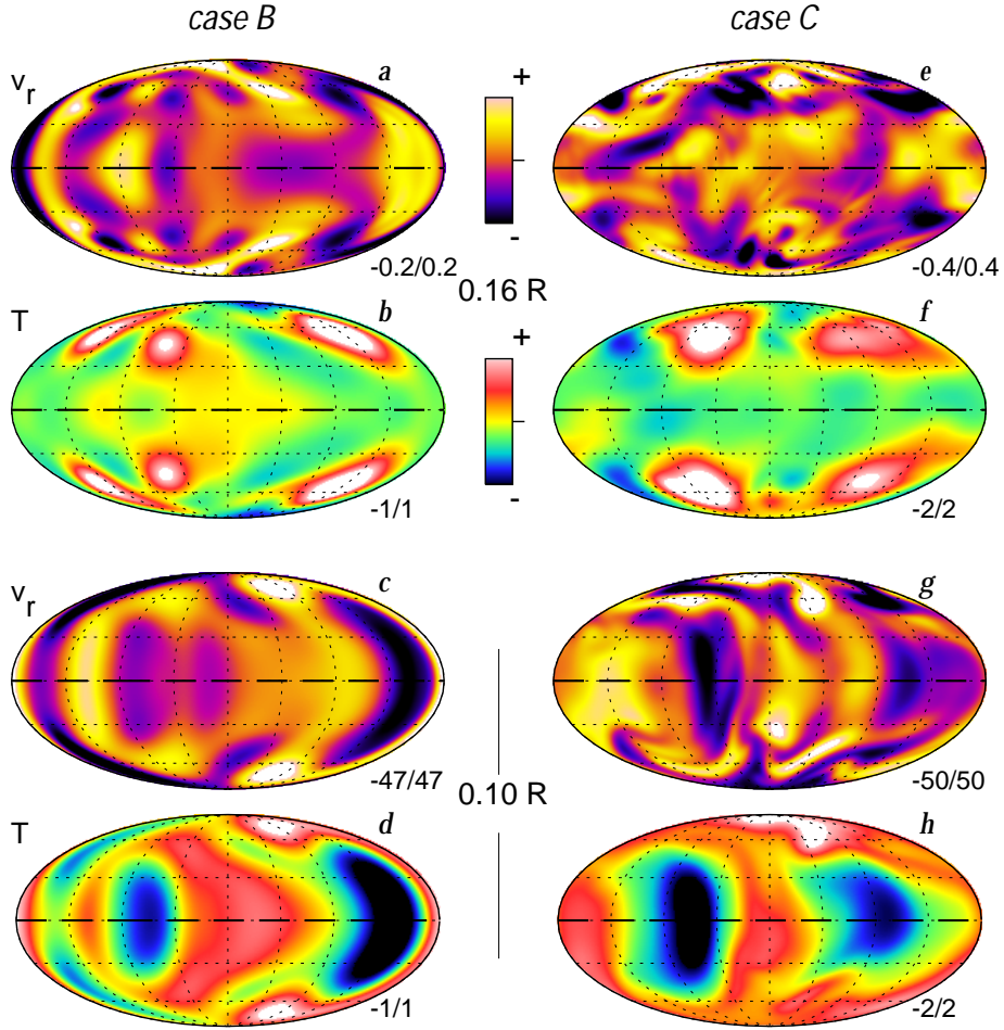
Fig. 3.— Global mappings of radial velocities ( v_r ) and associated temperature fluctuations ( T ) at one instant in time for the laminar case B (left column) and the more complex case C (right column), shown in Mollweide projection with the dashed horizontal line designating the equator. Two depths are sampled, with the lower panels exhibiting v_r and T within the convective core (at r = 0.10R ) and the upper panels within the region of overshooting (at r = 0.16R ). One color rendering is used for v_r , and another for T , with the maximum and minimum amplitudes for each field (in \text{m s}^{-1} and K) indicated next to each panel.
