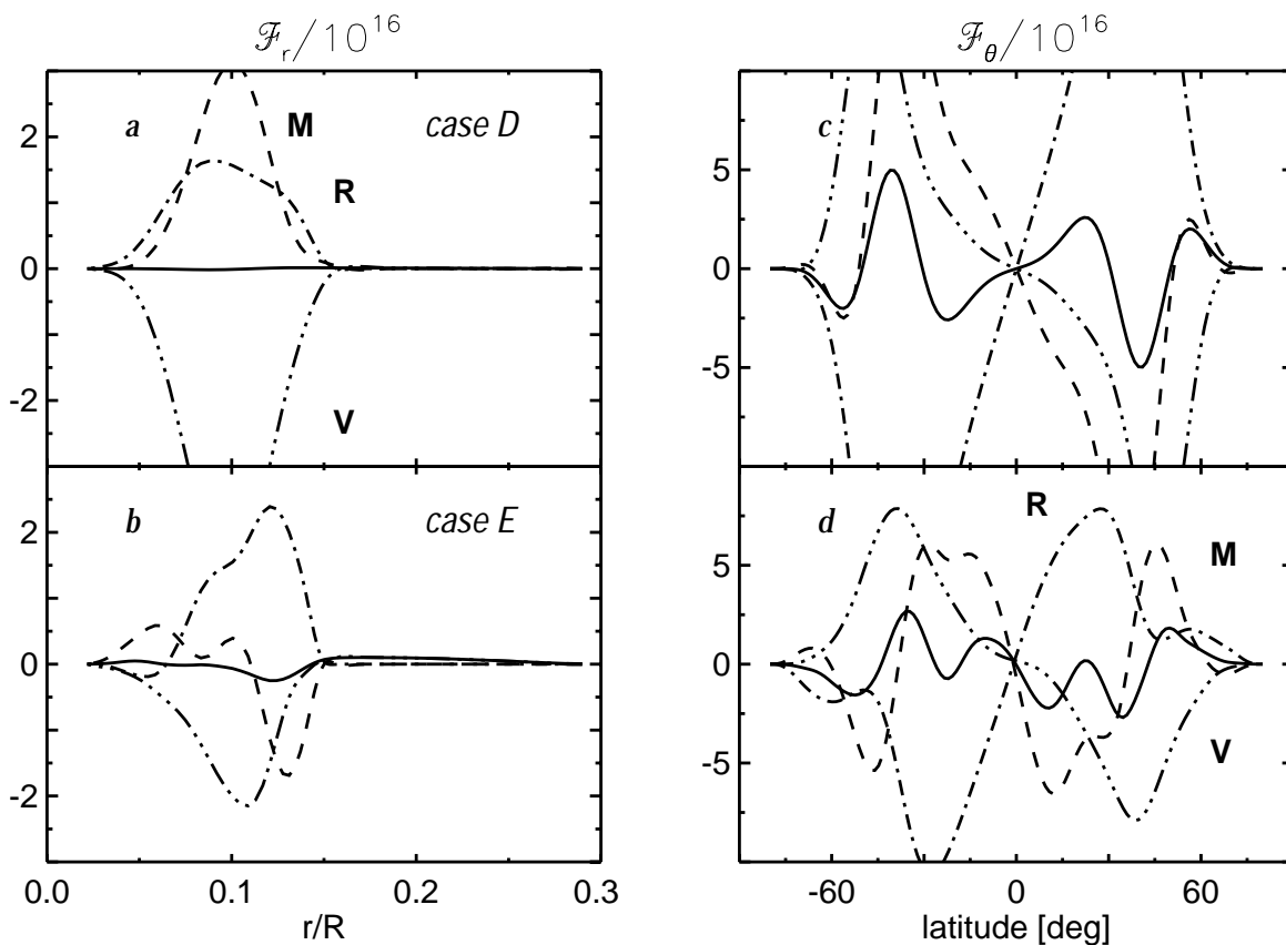
Fig. 15.— Time average of the latitudinal integral of the angular momentum flux \mathcal{F}_r (left panels) and of the radial integral of the angular momentum flux \mathcal{F}_\theta (right panels) for cases D (upper row) and E (lower row). The time intervals used in forming the averages were 670 days for case D and 620 days for case E. The fluxes have been decomposed into their viscous (V), Reynolds stress (R), and meridional circulation (M) components, and the solid curves represent the total fluxes. Positive quantities represent fluxes radially outward, or latitudinally from north to south.
