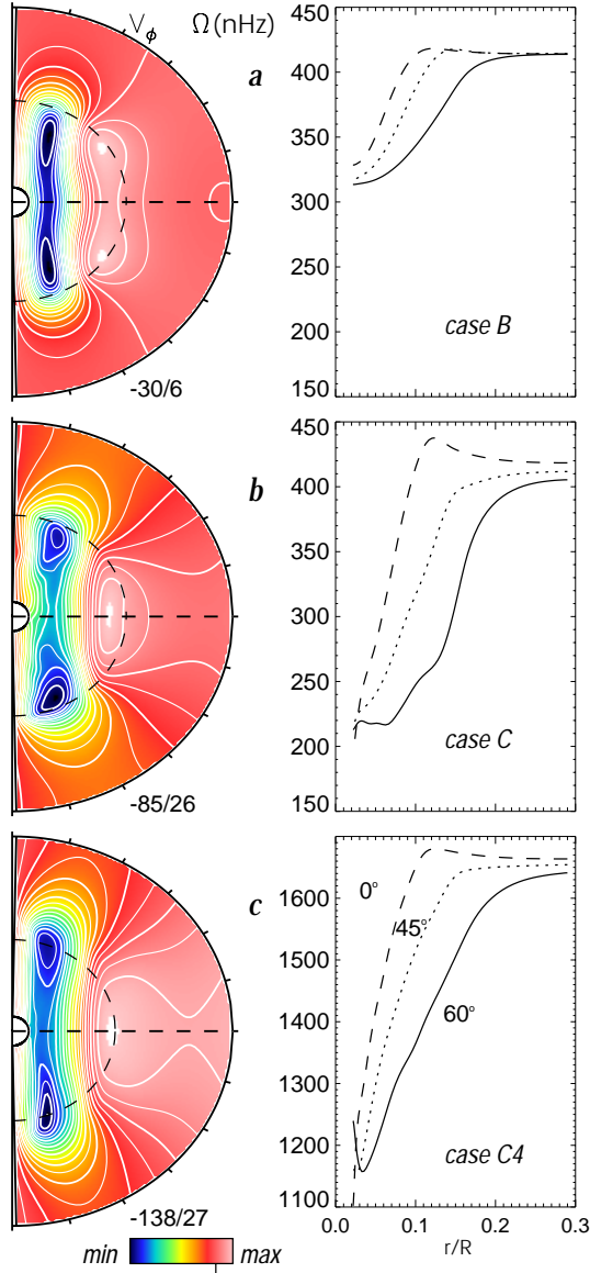
Fig. 6.— Strong differential rotation established by the convection in the three cases B, C, and C4. Shown are the azimuthal velocity \hat{v}_\phi as contour plots in radius and latitude (left panels, with dashed line denoting equator), and the angular velocity \hat{\Omega} with proportional radius for three latitudinal cuts (right panels); both \hat{v}_\phi and \hat{\Omega} are averaged in time (all over intervals of roughly 110 days) and longitude. Maxima and minima of \hat{v}_\phi (in \text{m s}^{-1} ) are indicated. Cases B and C (upper, middle panels) are rotating at the solar rate (414 nHz), and case C4 (lower panels) rotates fourfold faster. Greater angular velocity contrasts are achieved in the more complex flows of case C, C4 (b,c) than in the laminar case B (a), in all cases involving a central column of slowness.
