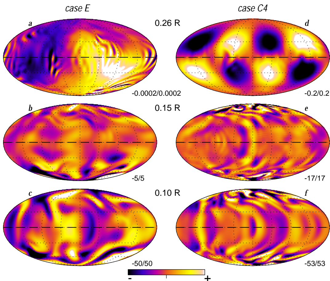
Fig. 9.— The excitation of gravity waves in the radiative envelope for cases E (left) and C4 (right), shown in global mappings of radial velocity v_r at one instant in time (top panels, sampling r = 0.26R ). The associated convective flows are also shown within the overshoot region (middle panels, r = 0.15R ) and in the convective core (lower panels, r = 0.10R ). For case E, gravity waves of small amplitude (scaling indicated) are visible in (a) as weak ripples in the largely quiescent radiative zone. For case C4, the waves appear in (d) as a prominent global resonance of greater amplitude.
