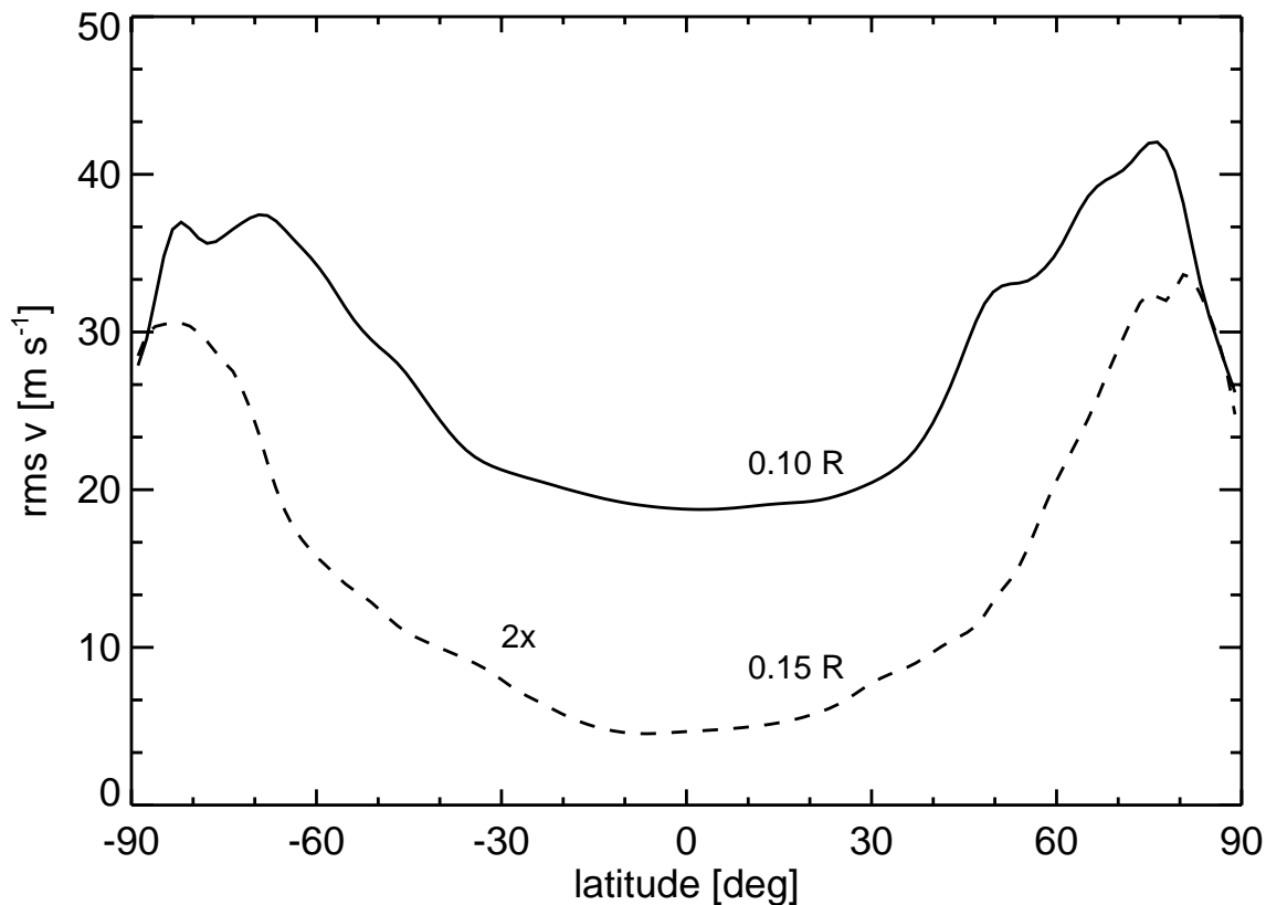
Fig. 12.— Variation with latitude of the root-mean-square of radial velocities \tilde{v}_r in case C within both the convective core ( r = 0.10R ) and the region of overshooting ( r = 0.15R ), averaged over 180 days. The latter velocities have been multiplied by a factor of two for visibility. Radial velocities are highest near the poles, and lowest near the equator, owing partly to the deflection of outward motions by the Coriolis forces in these rotating domains. The prolate geometry of the convective core appears to arise from such latitudinal variation of v_r .
