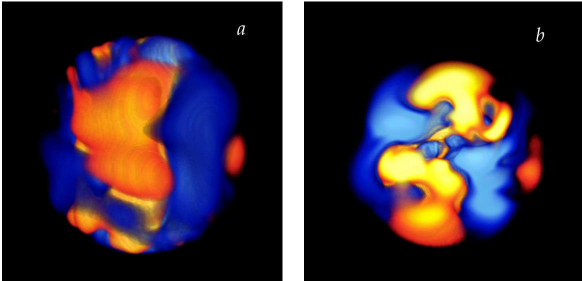
Fig. 2.— Radial velocity at one instant in time for case E, using volume rendering of flow structure ( a ) near the outer boundary of the prolate convective core, with the rotation axis oriented vertically, and ( b ) near the equatorial plane viewed from above. Upflows (radially outward) are rendered as yellow/red tones; downflows are bluish.
