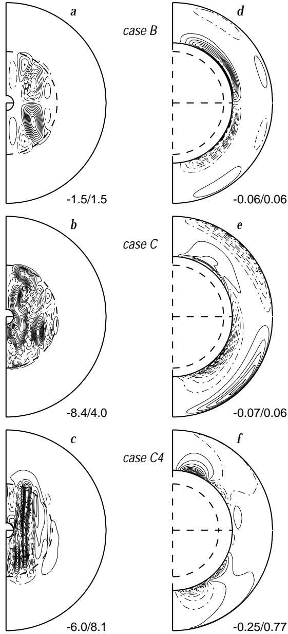
Fig. 14.— Time-averaged streamfunctions of meridional mass flux for cases B (upper panels), C (middle), and C4 (lower), displayed for the whole domain (left column) and at much amplified scaling for the outer portion of the radiative zone only (right). The time intervals used in the averaging are all of order 110 days. Solid lines denote counter-clockwise flow, dashed lines clockwise. The associated maximum and minimum velocities for \tilde{v}_\theta (in \text{m s}^{-1} ) are indicated.
