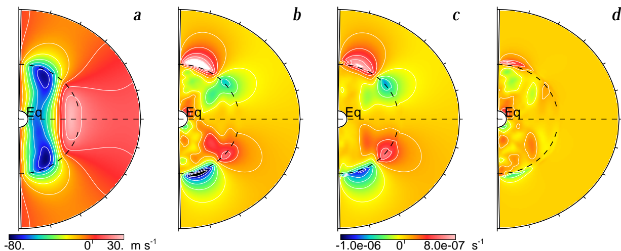
Fig. 16.— Temporal (640-day) and longitudinal averages for case E showing (a) the longitudinal velocity \hat{v}_\phi , (b) d\hat{v}_\phi/dz , (c) the baroclinic term in the meridional force balance, and (d) the difference between the latter two. The same color scale is used in (b), (c), and (d). Near the interface between the convective core and the radiative envelope, baroclinic effects account for much of the differential rotation. Within the bulk of the prolate convective core, Reynolds and viscous stresses have a significant role in driving those zonal flows.
